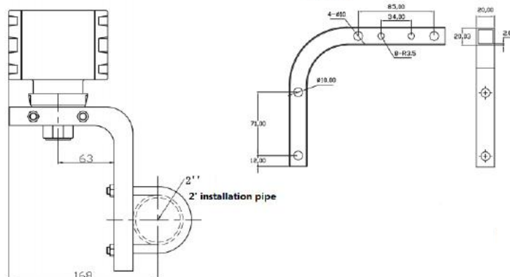
WinSMART™ Pressure Transmitter (threaded interface) overall dimensions (unit: mm)
